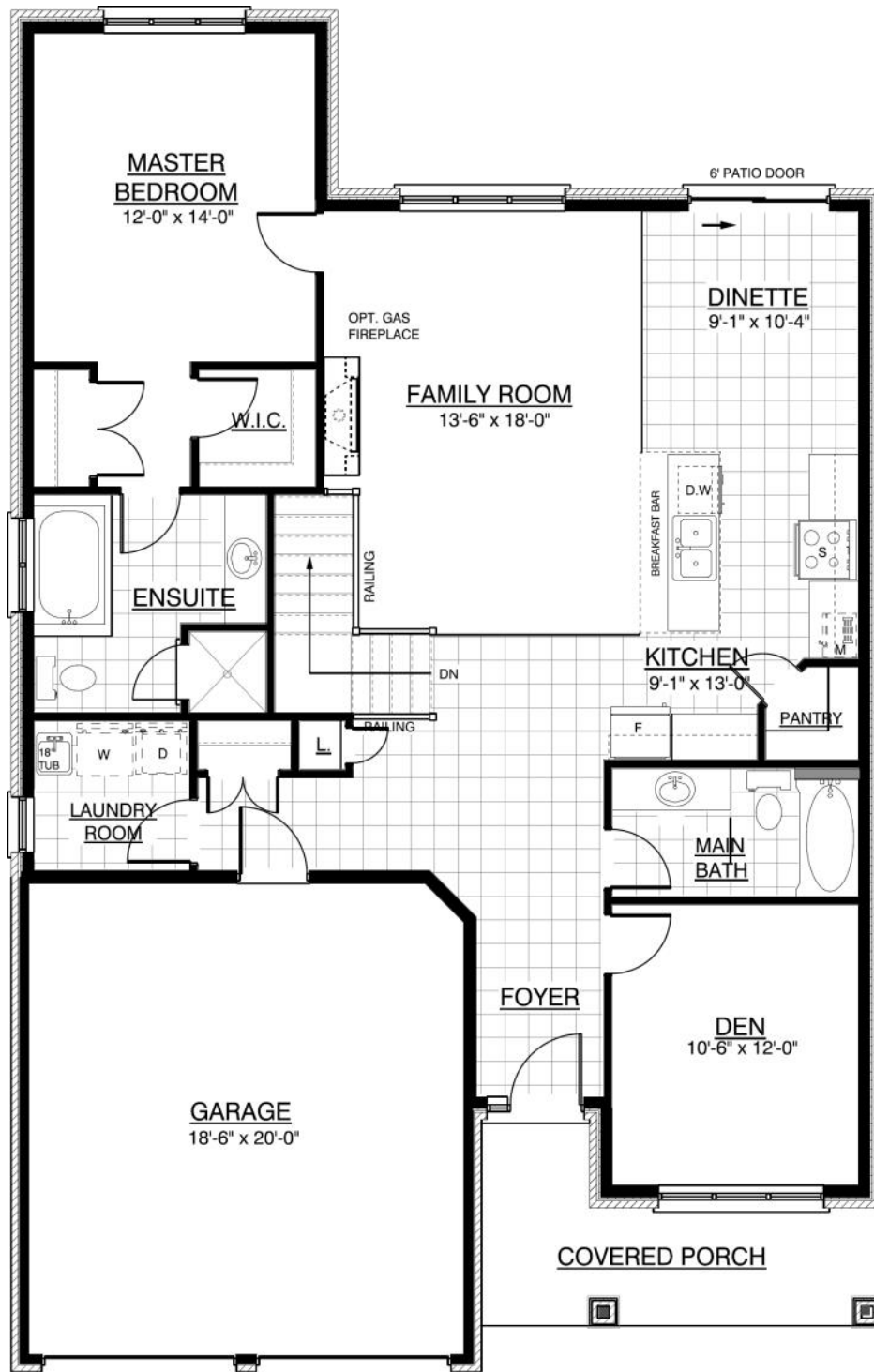
Main Floor Plan "A" - 1,415 sqft
