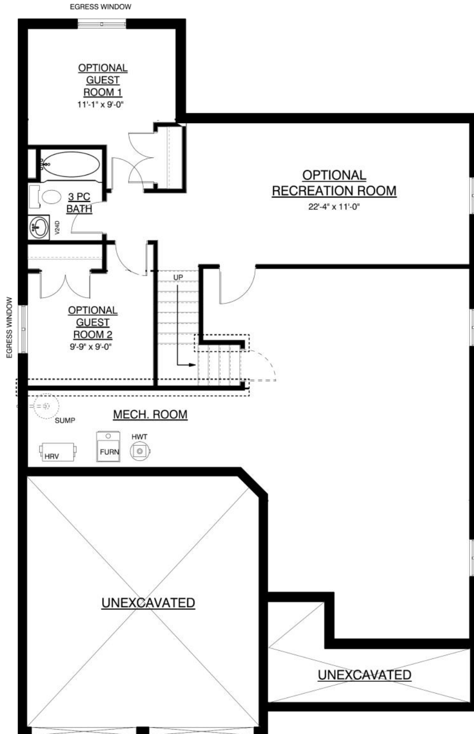
Optional Finished Basement Plan - 600 sqft finished area
