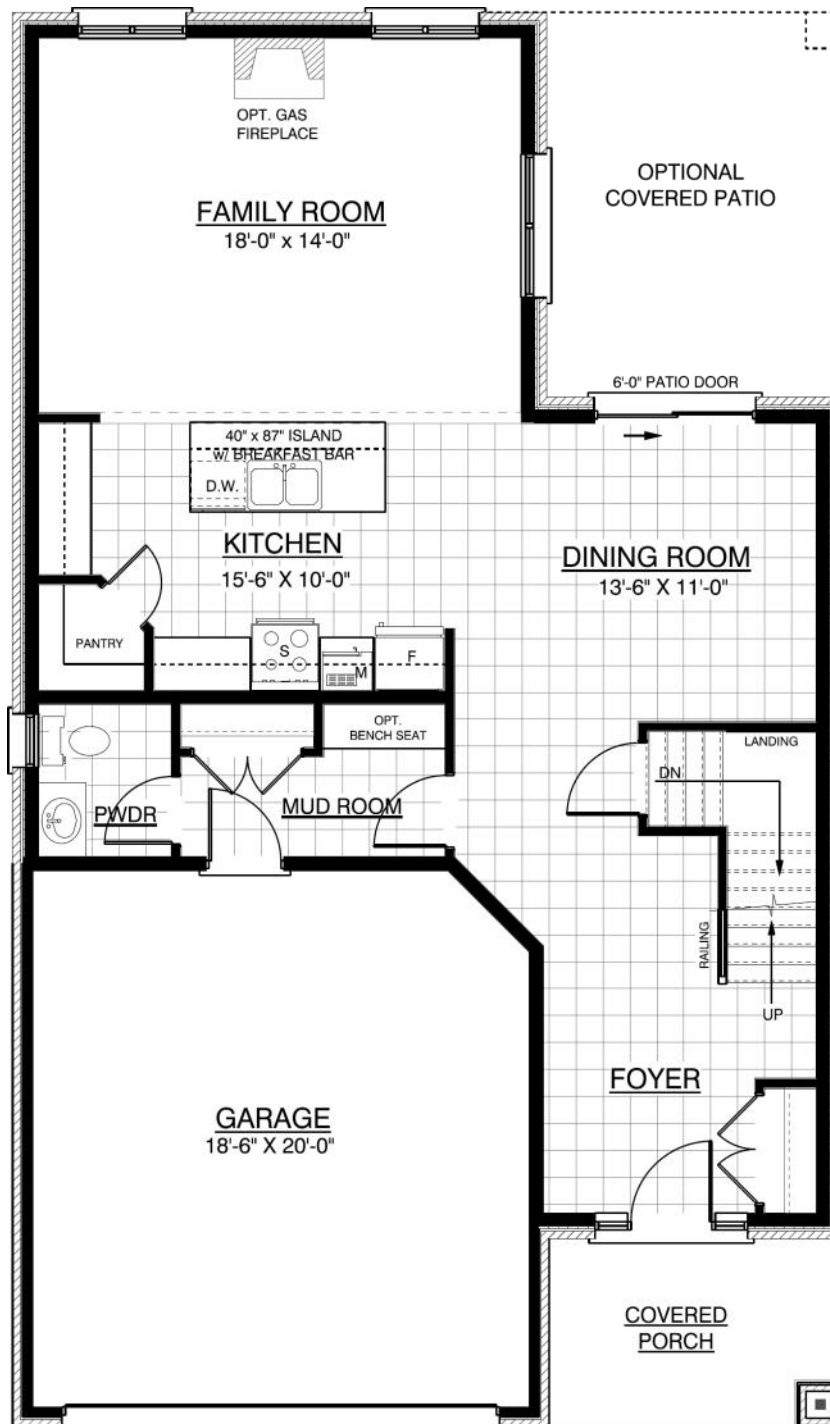
Main Floor Plan - 988 sqft
