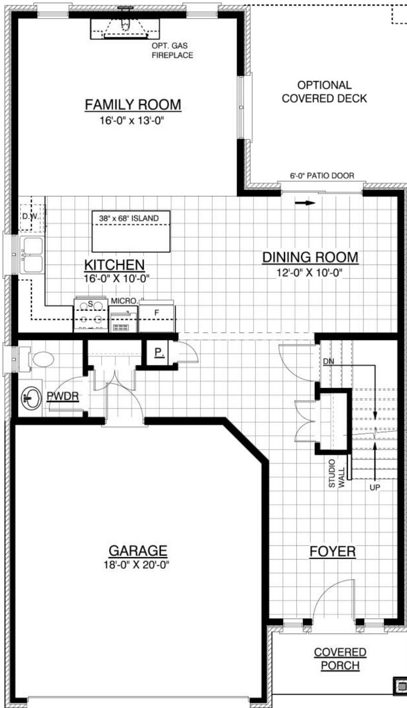
Main Floor Plan - 918 sqft
