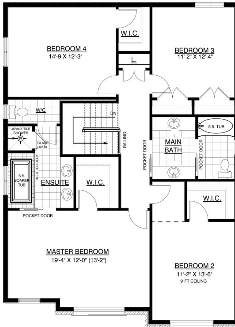
Upper Floor Plan - 1,326 sqft
