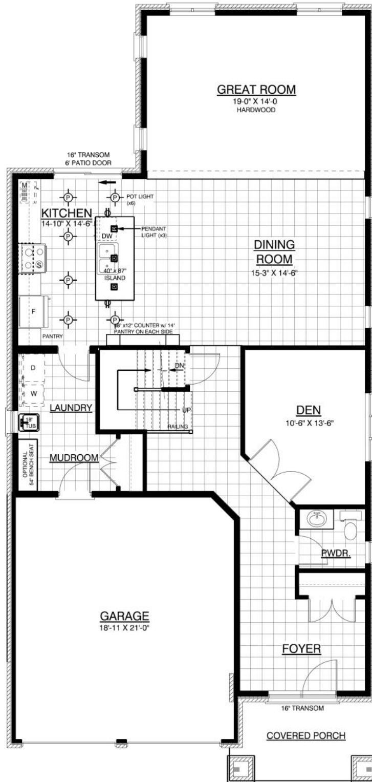
Main Floor Plan - 1,429 sqft
