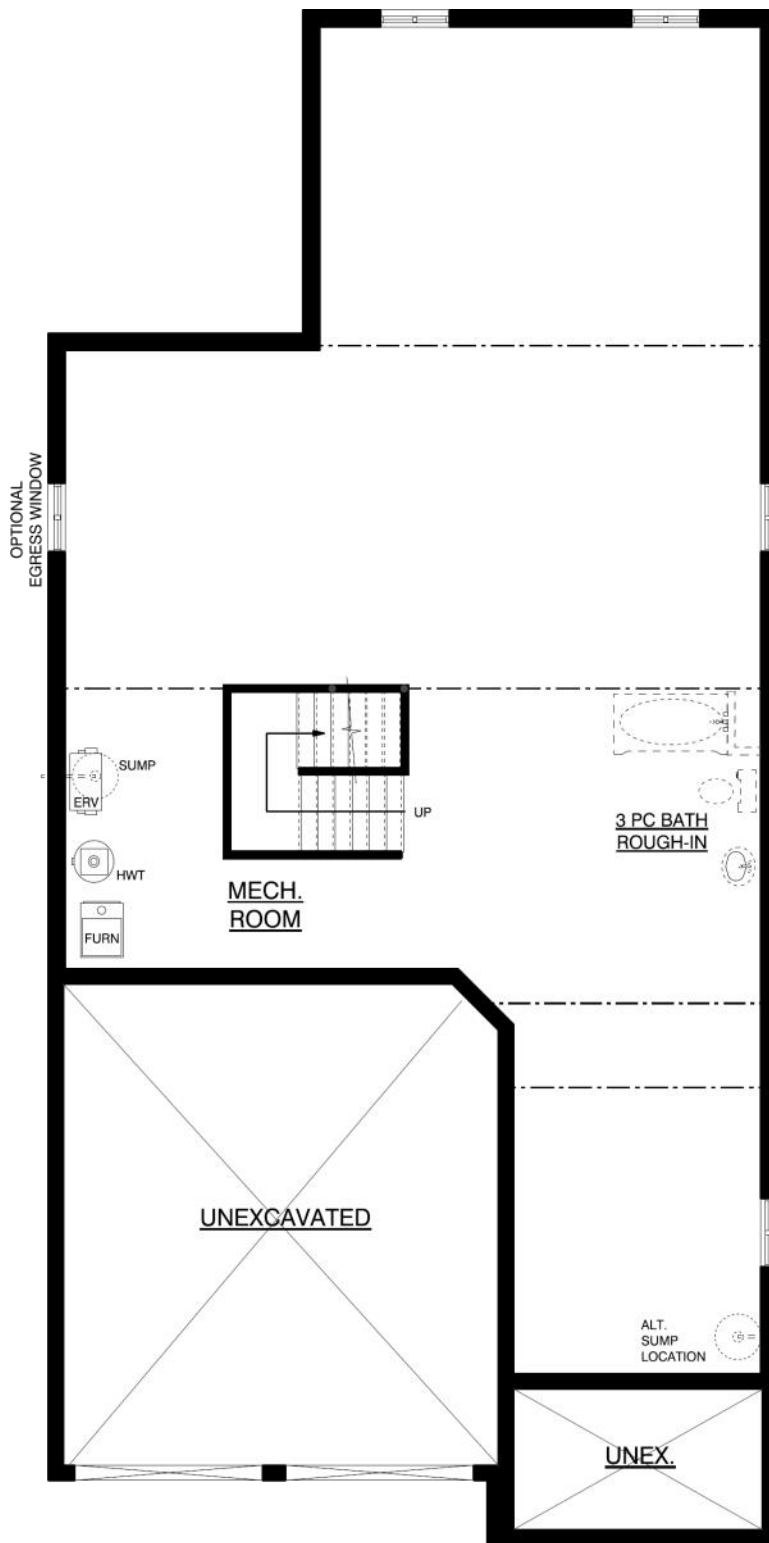
Basement Plan
