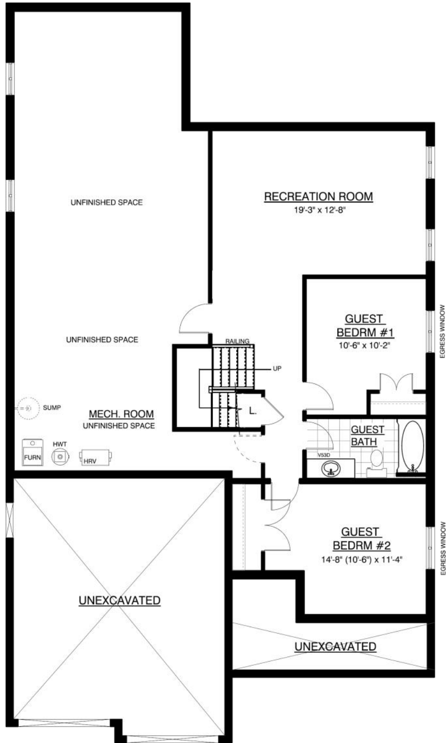
Optional Finished Basement Plan - 760 sqft finished area
