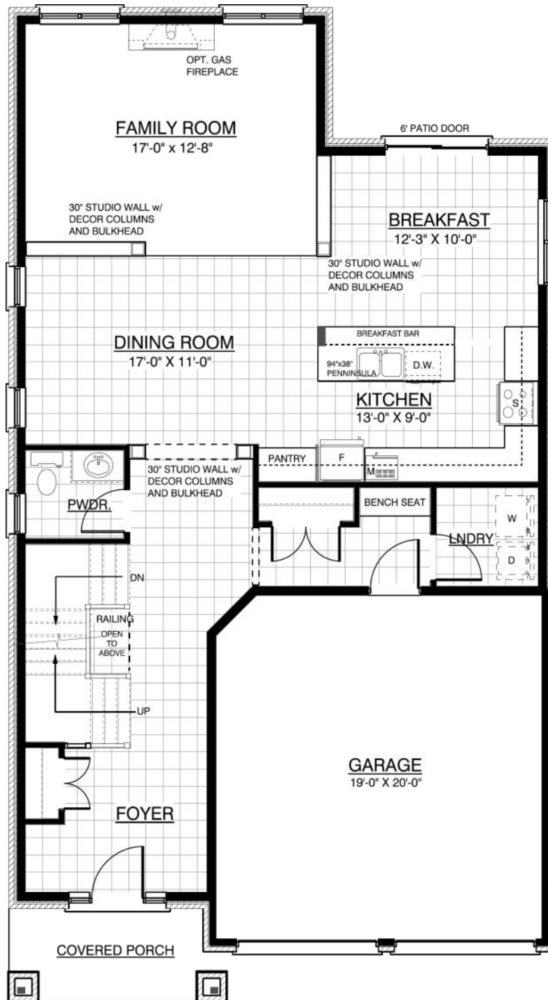
Main Floor Plan - 1,208 sqft
