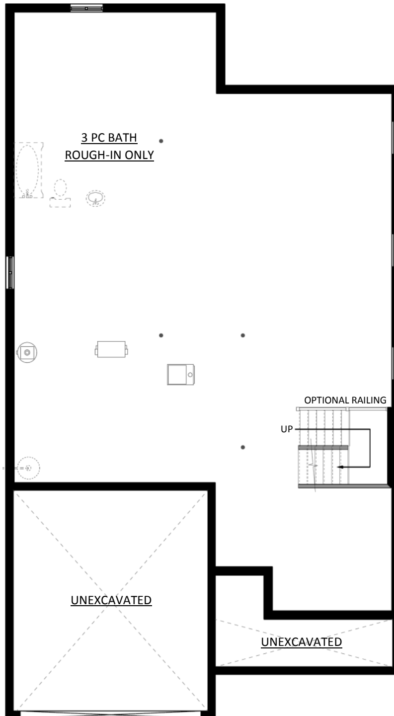
Standard Unfinished Basement Plan
