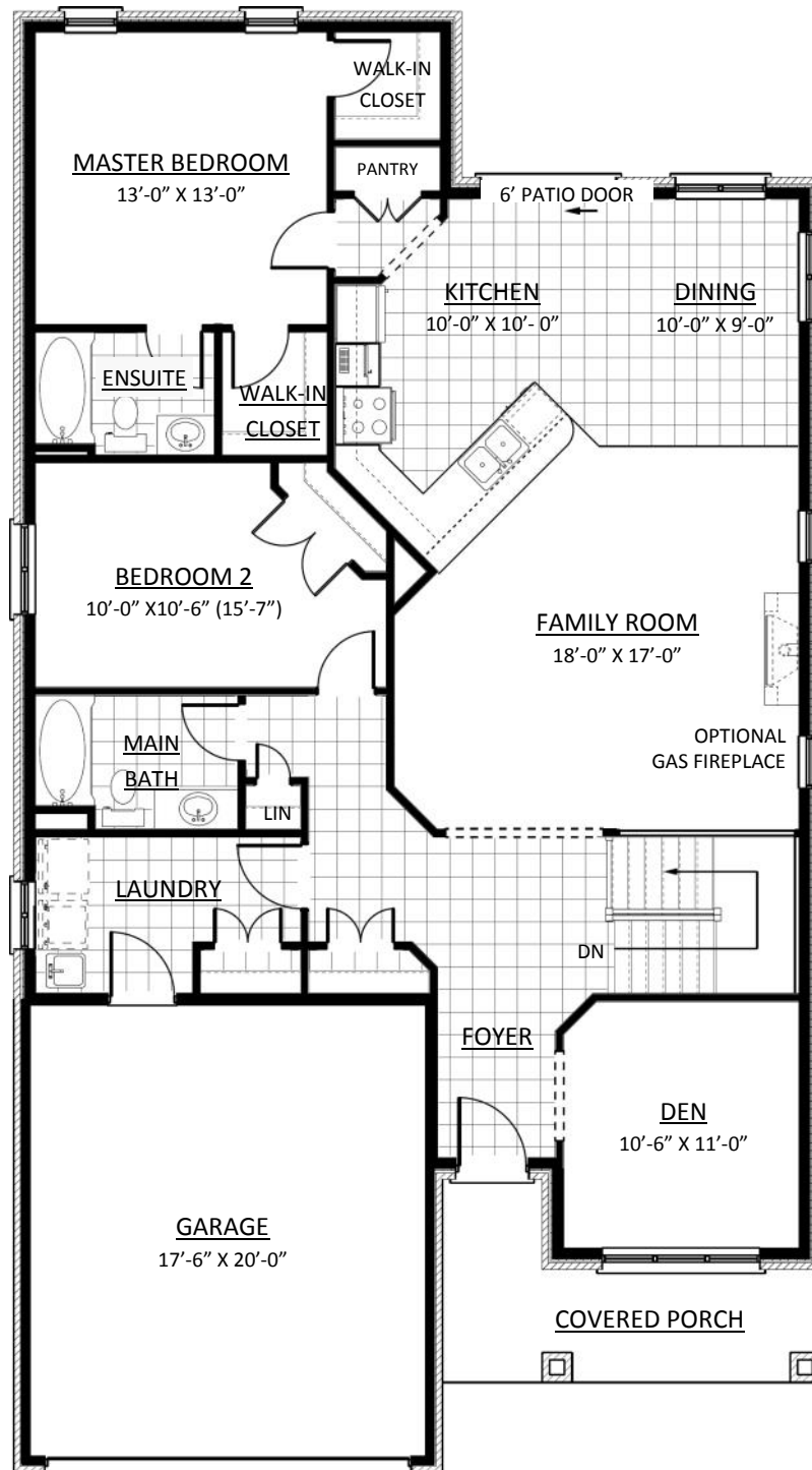
Main Floor Plan - 1,645 sqft
