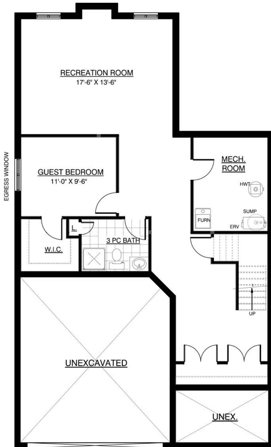
Optional Finished Basement Plan - 830 sqft finished area
